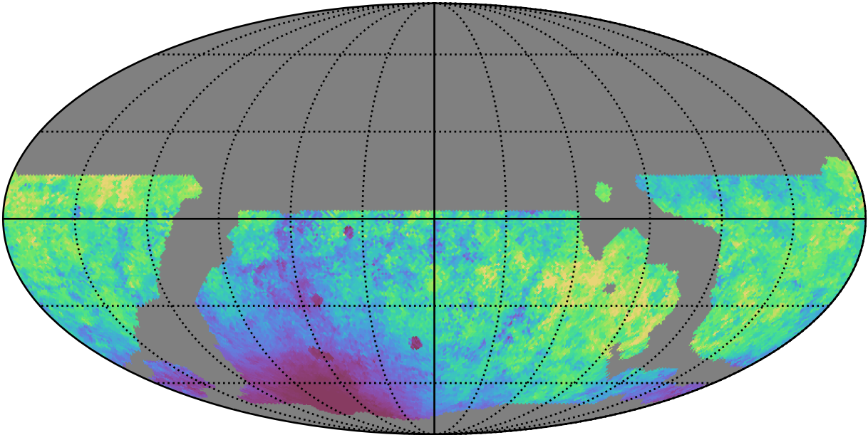
weather_cloudso8v3.4_10yrs WFD r band: Median moonDistance
