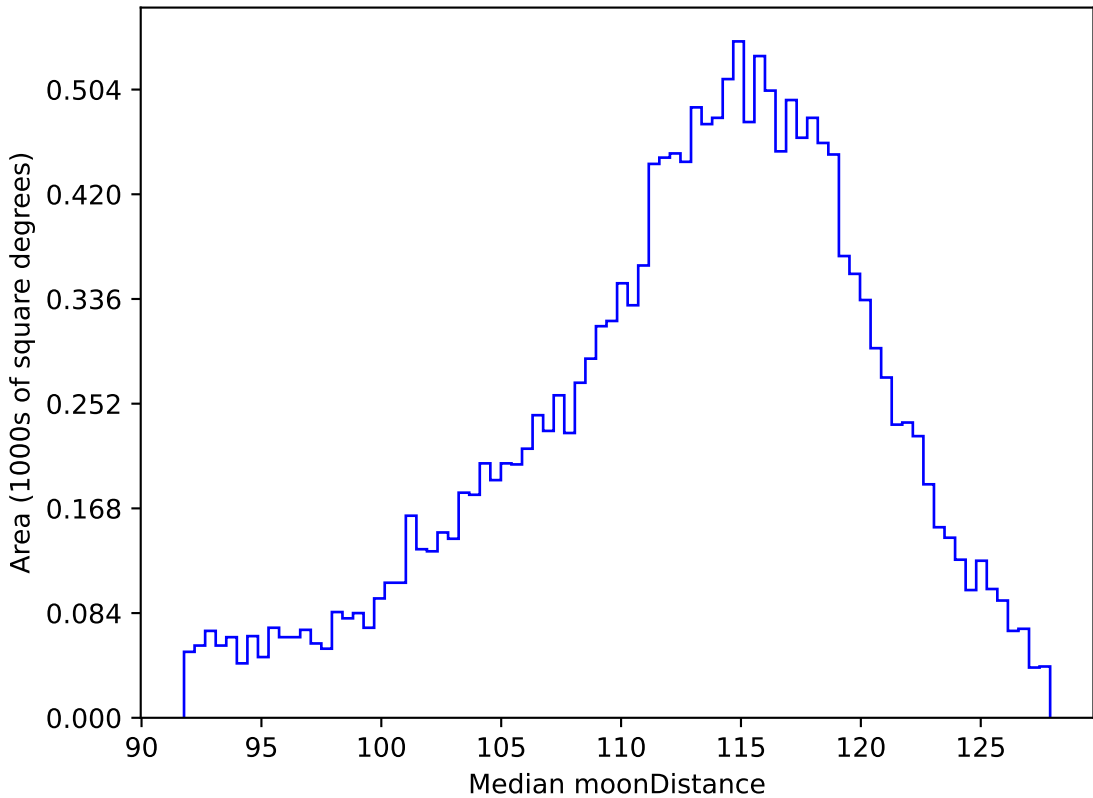
weather_cloudso8v3.4_10yrs WFD r band: Median moonDistance
