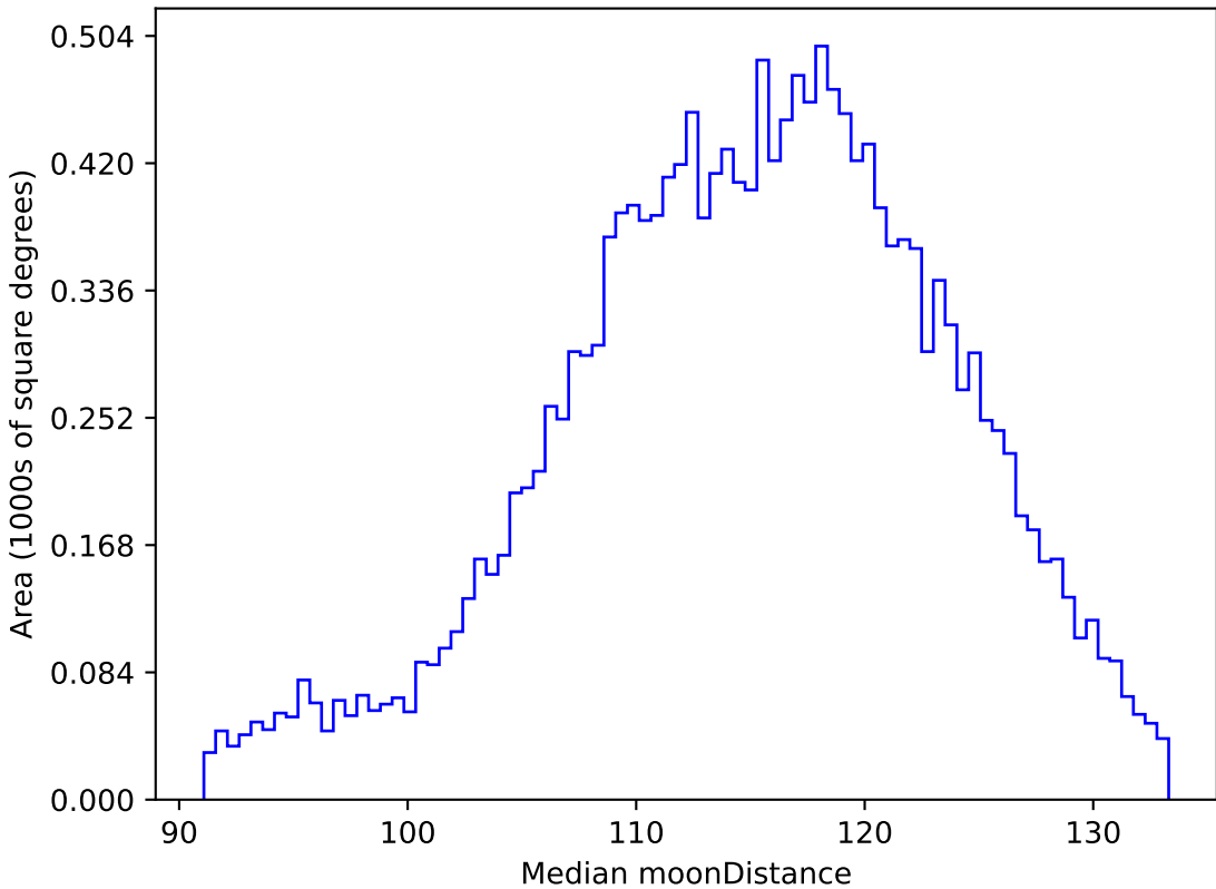
weather_cloudso8v3.4_10yrs WFD g band: Median moonDistance
