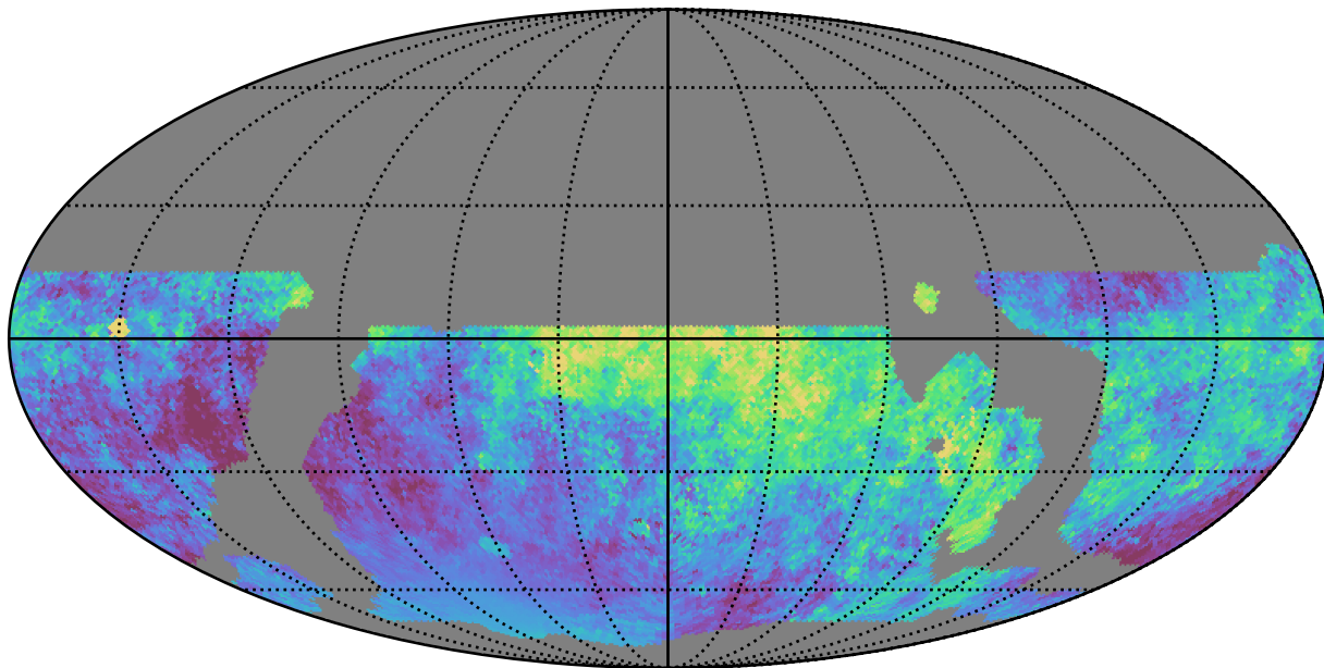
weather_cloudso8v3.4_10yrs WFD all bands: Median moonDistance
