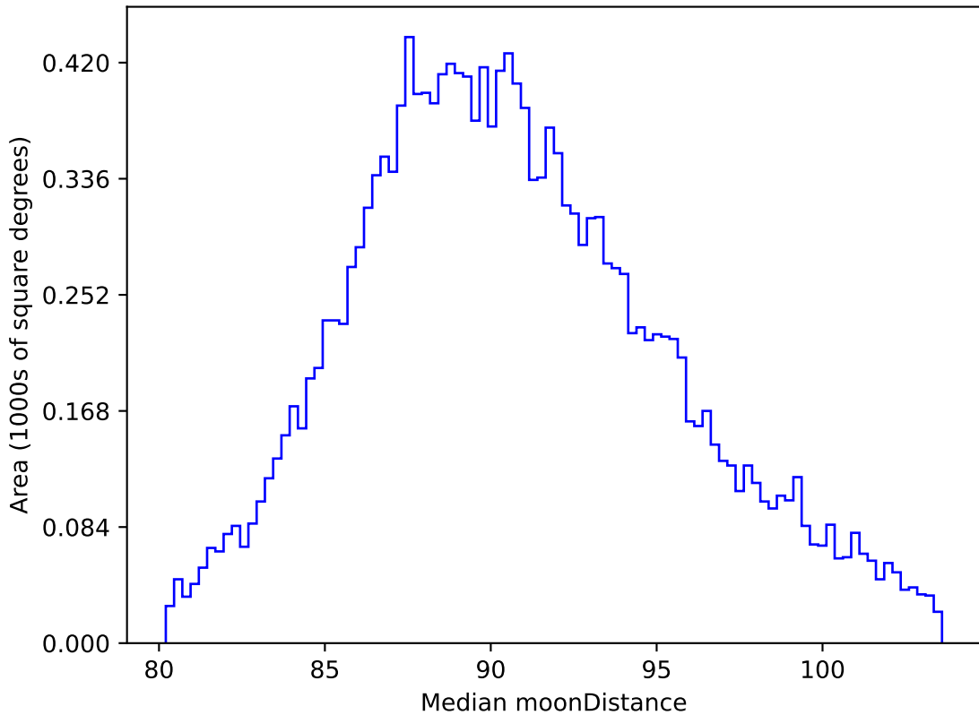
weather_cloudso8v3.4_10yrs WFD all bands: Median moonDistance
