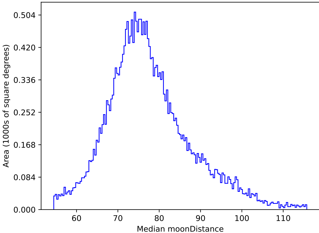
weather_cloudso8v3.4_10yrs All sky z band: Median moonDistance
