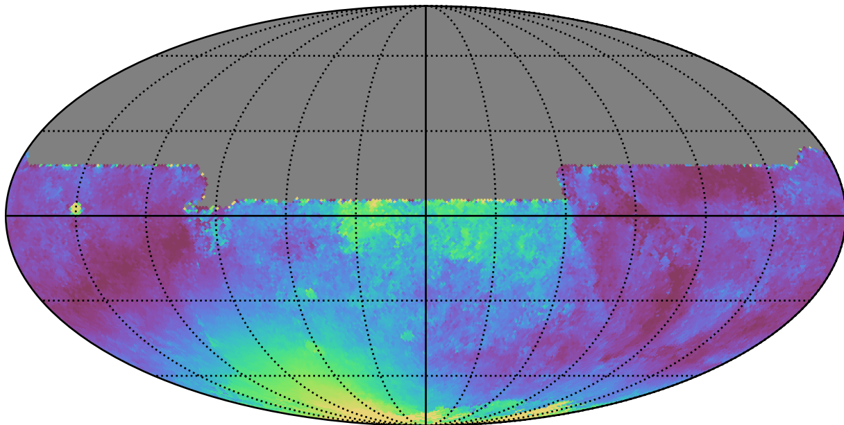
weather_cloudso8v3.4_10yrs All sky y band: Median moonDistance
