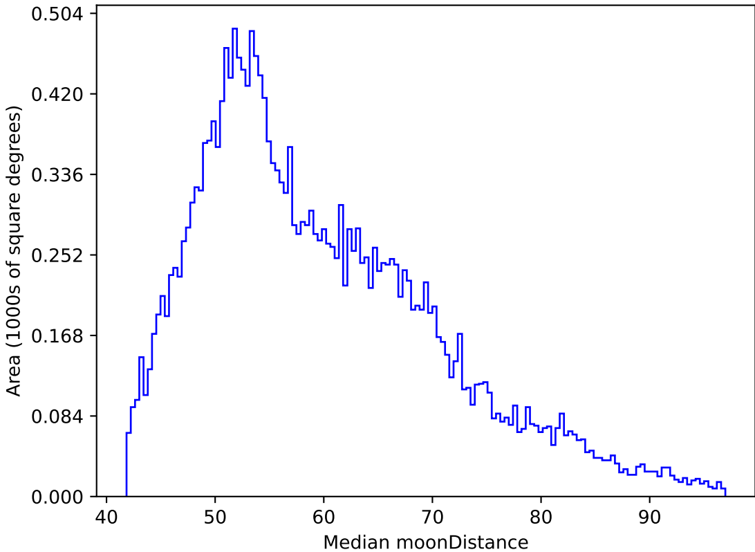
weather_cloudso8v3.4_10yrs All sky y band: Median moonDistance
