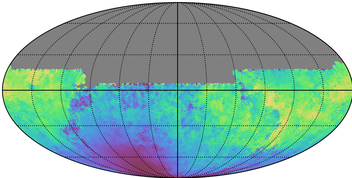
weather_cloudso8v3.4_10yrs All sky u band: Median moonDistance
