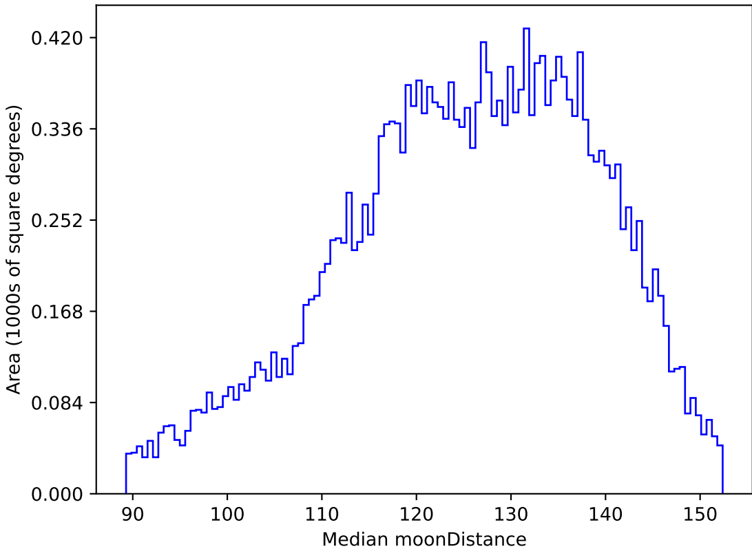
weather_cloudso8v3.4_10yrs All sky u band: Median moonDistance
