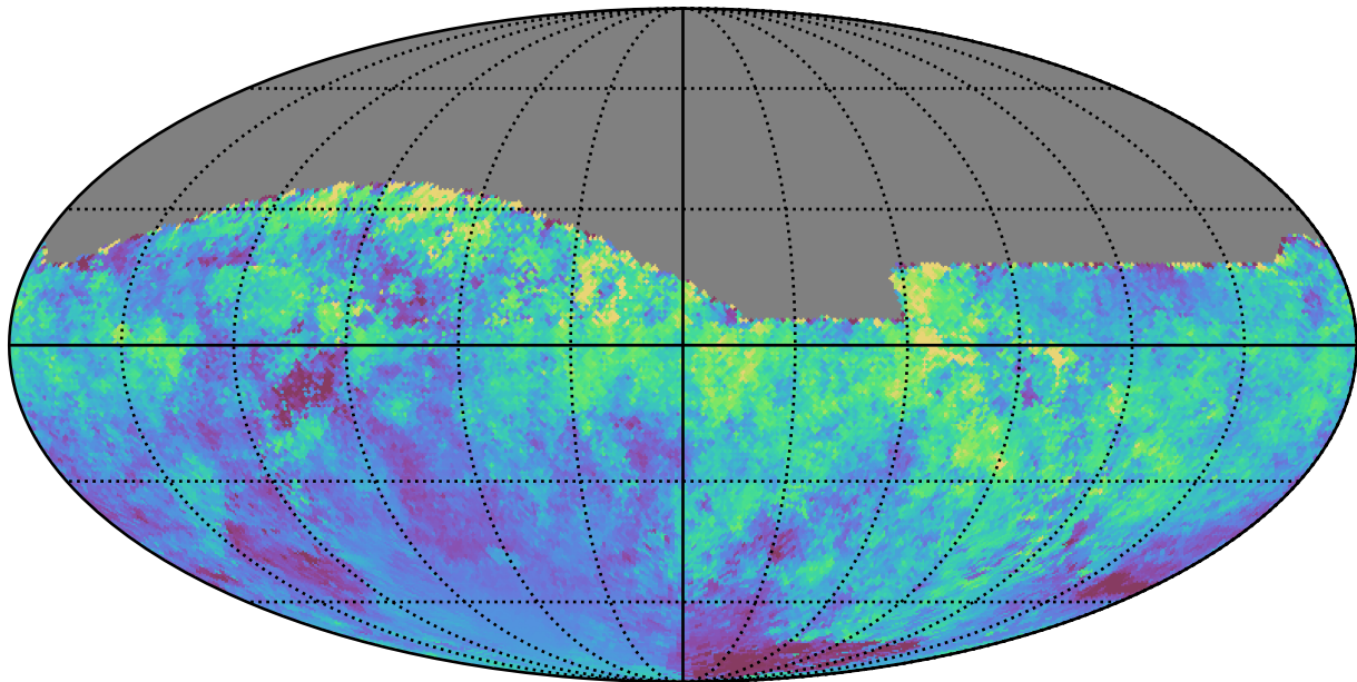
weather_cloudso8v3.4_10yrs All sky i band: Median moonDistance
