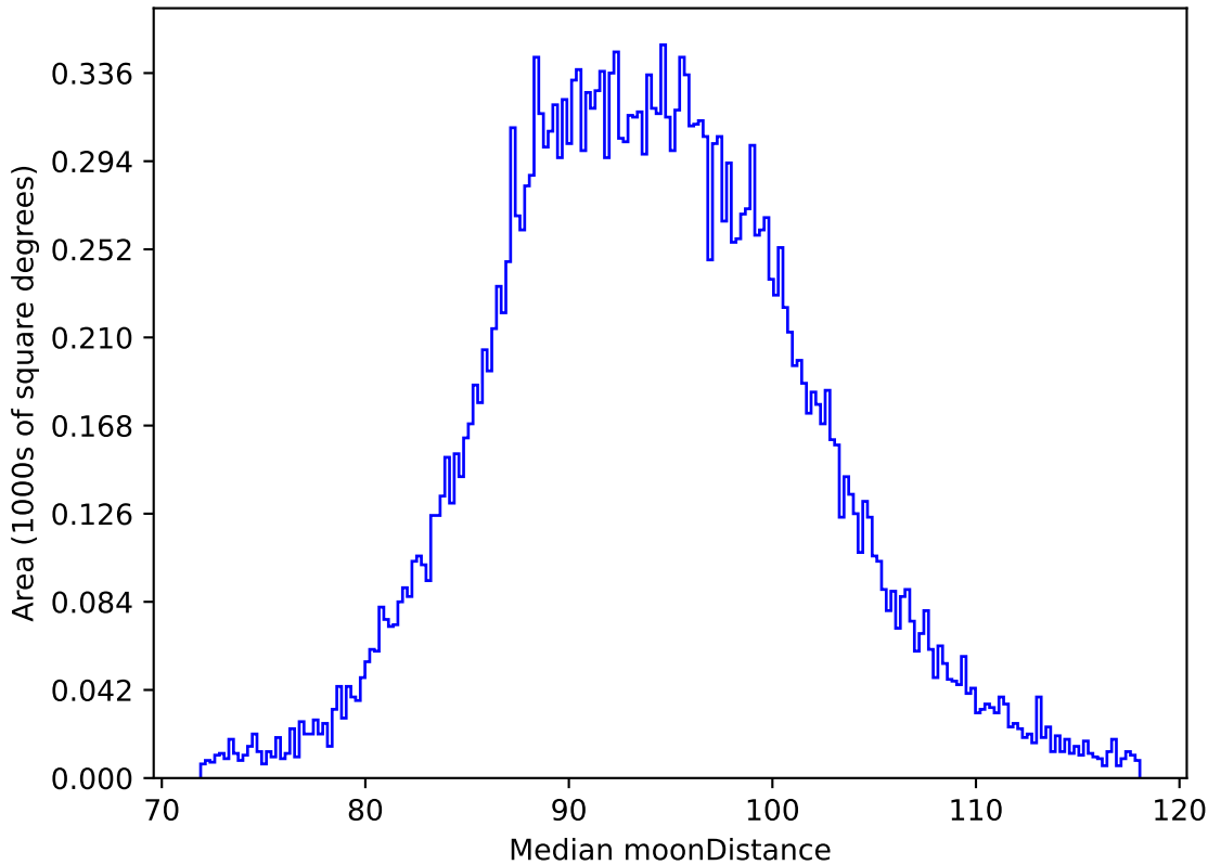
weather_cloudso8v3.4_10yrs All sky i band: Median moonDistance
