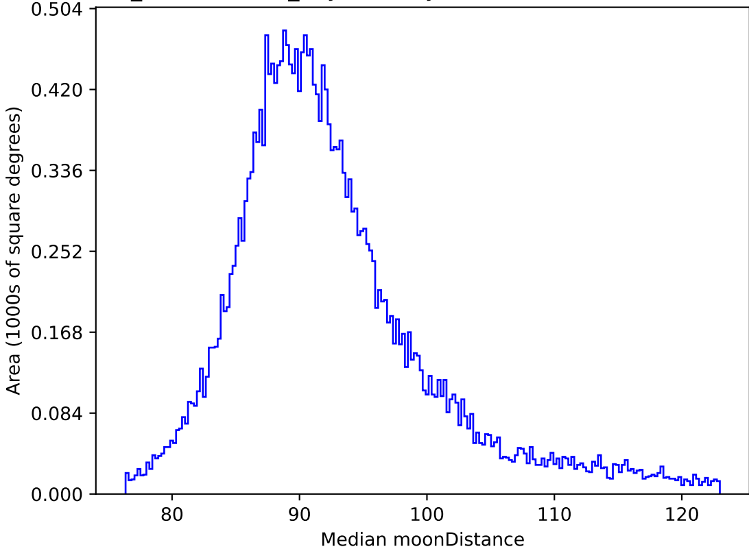
weather_cloudso8v3.4_10yrs All sky all bands: Median moonDistance
