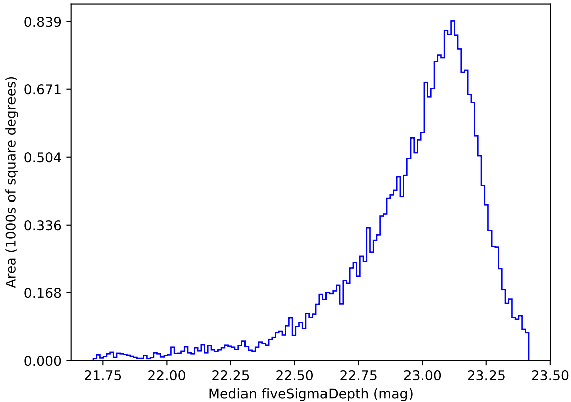
weather_cloudso8v3.4_10yrs Yr 1 z band: Median fiveSigmaDepth
