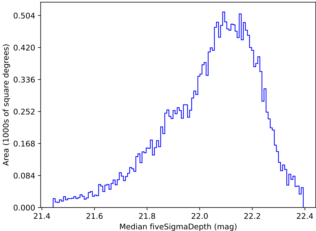
weather_cloudso8v3.4_10yrs Yr 1 y band: Median fiveSigmaDepth
