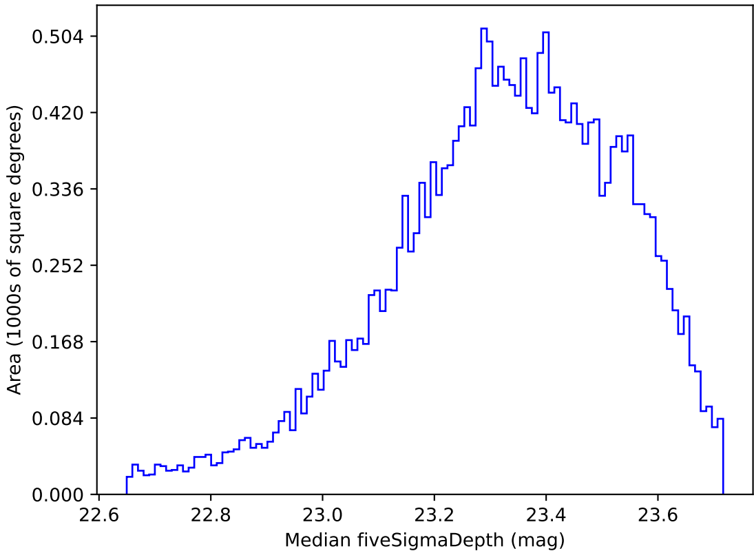
weather_cloudso8v3.4_10yrs Yr 1 u band: Median fiveSigmaDepth
