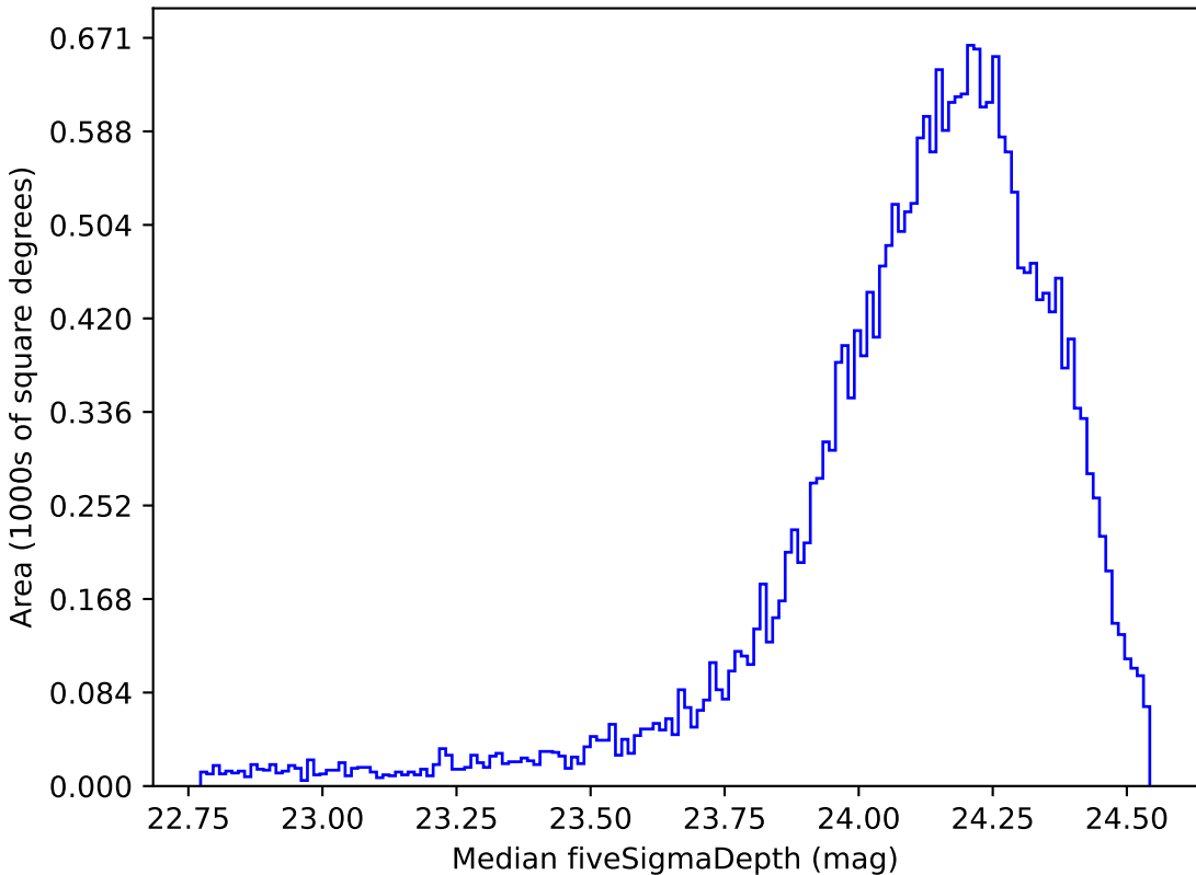
weather_cloudso8v3.4_10yrs Yr 1 r band: Median fiveSigmaDepth
