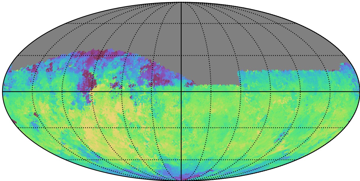
weather_cloudso8v3.4_10yrs Yr 1 i band: Median fiveSigmaDepth
