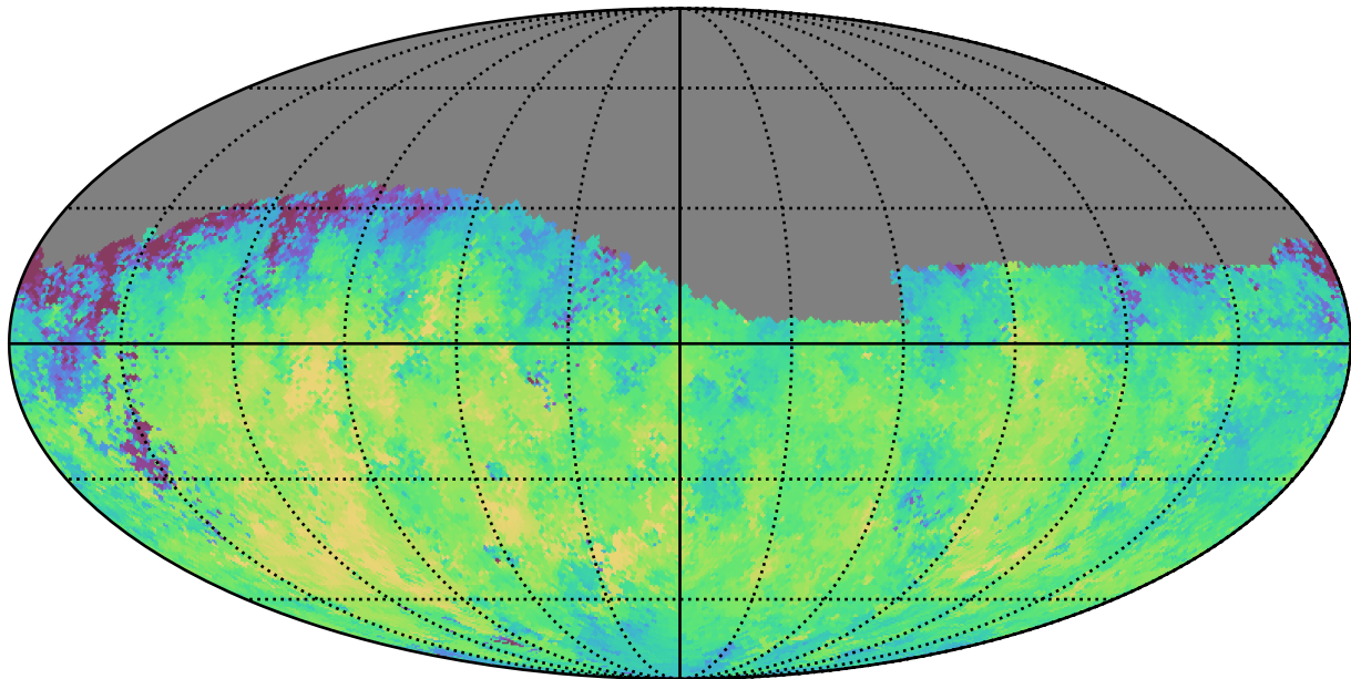
weather_cloudso8v3.4_10yrs Yr 1 g band: Median fiveSigmaDepth
