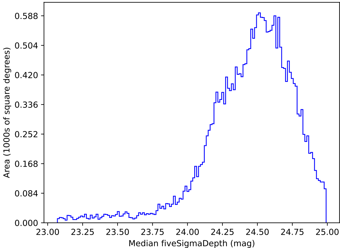
weather_cloudso8v3.4_10yrs Yr 1 g band: Median fiveSigmaDepth
