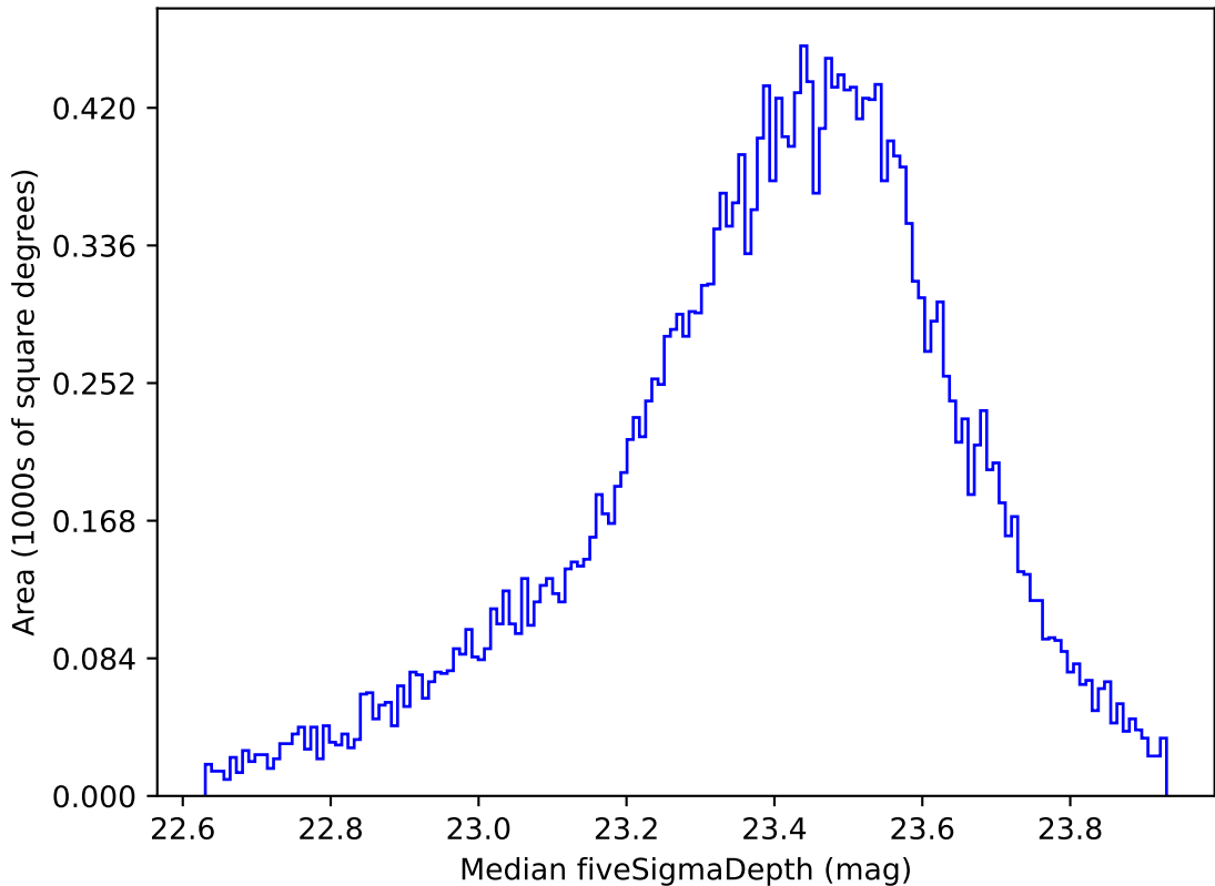
weather_cloudso8v3.4_10yrs Yr 1 all bands: Median fiveSigmaDepth
