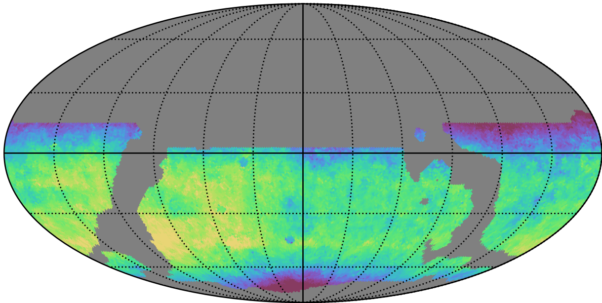
weather_cloudso8v3.4_10yrs WFD y band: Median fiveSigmaDepth
