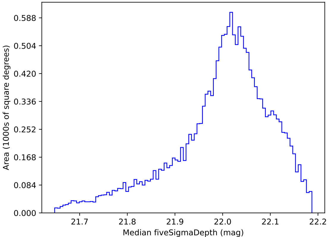
weather_cloudso8v3.4_10yrs WFD y band: Median fiveSigmaDepth
