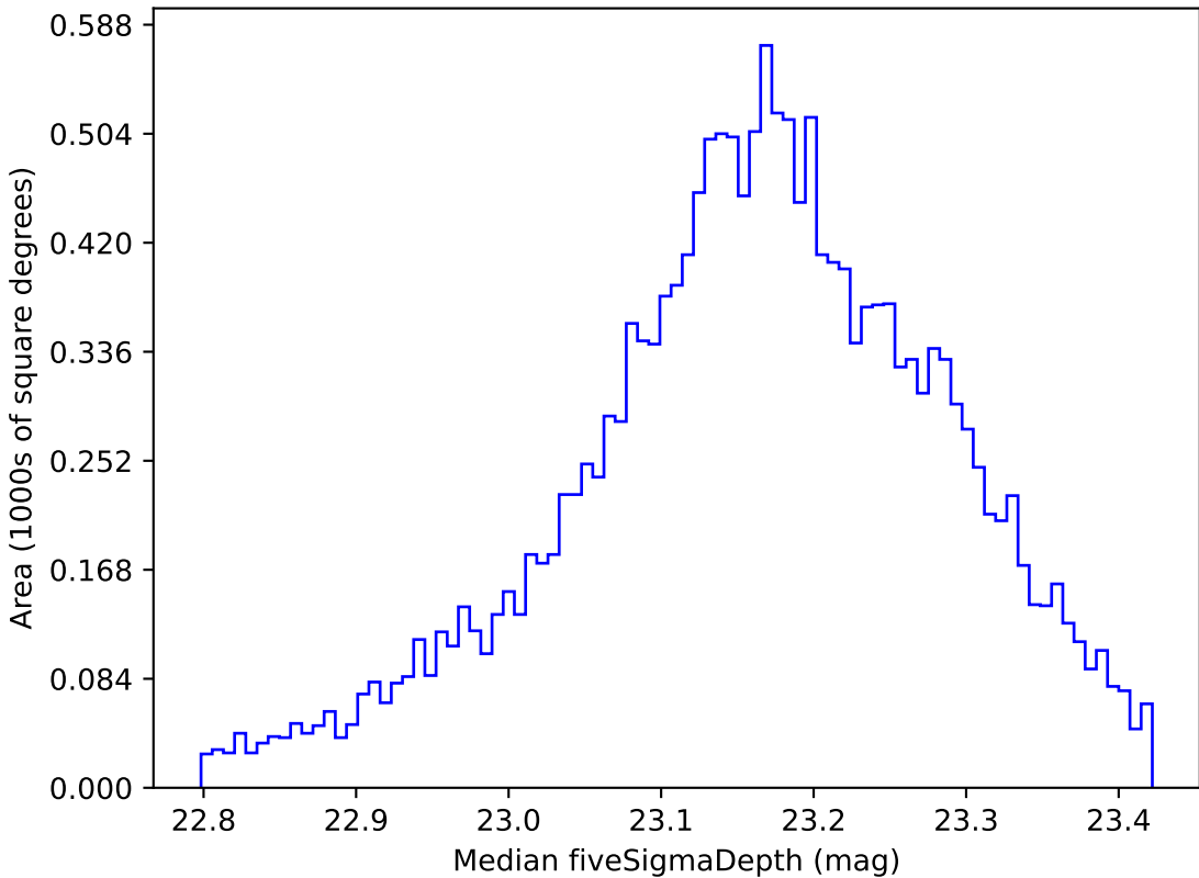
weather_cloudso8v3.4_10yrs WFD u band: Median fiveSigmaDepth
