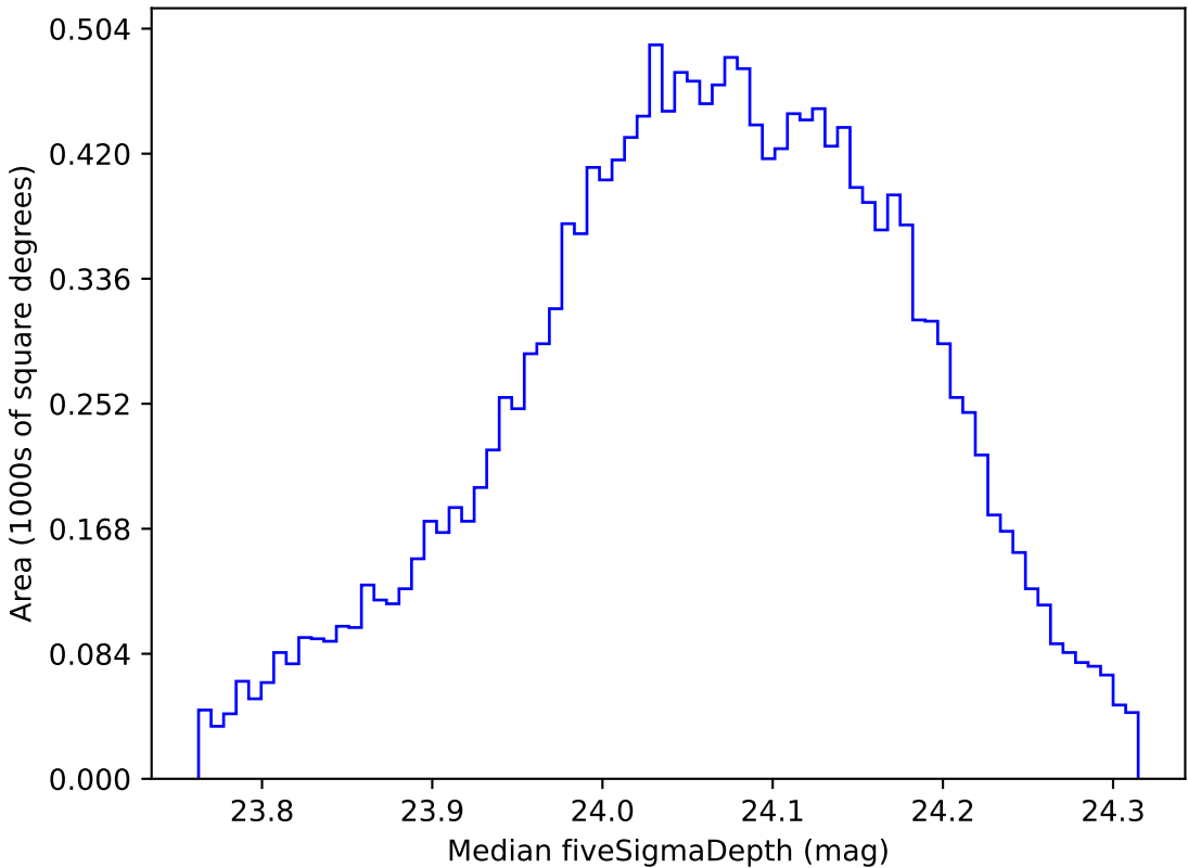
weather_cloudso8v3.4_10yrs WFD r band: Median fiveSigmaDepth
