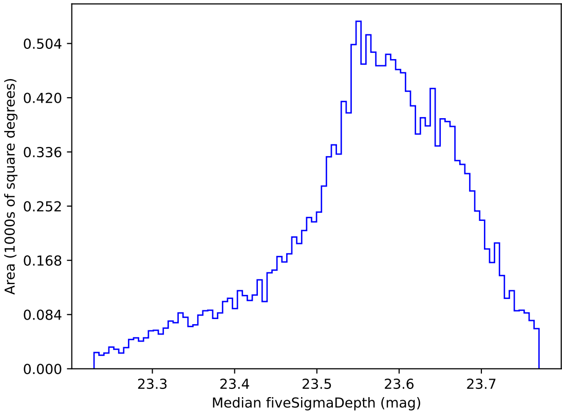
weather_cloudso8v3.4_10yrs WFD i band: Median fiveSigmaDepth
