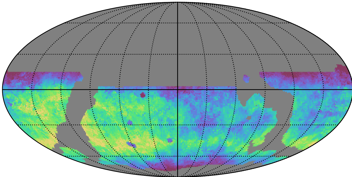
weather_cloudso8v3.4_10yrs WFD g band: Median fiveSigmaDepth
