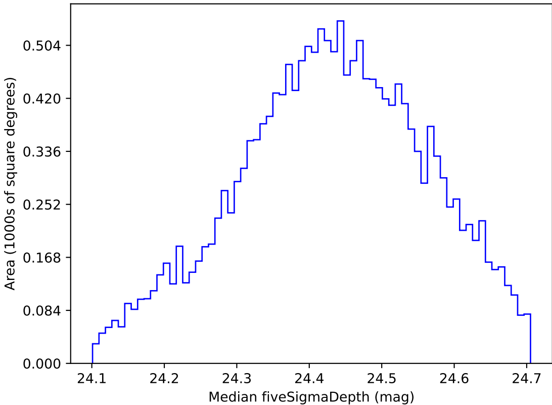
weather_cloudso8v3.4_10yrs WFD g band: Median fiveSigmaDepth
