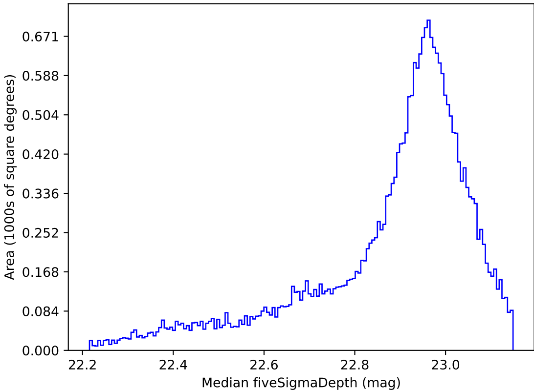
weather_cloudso8v3.4_10yrs All sky z band: Median fiveSigmaDepth
