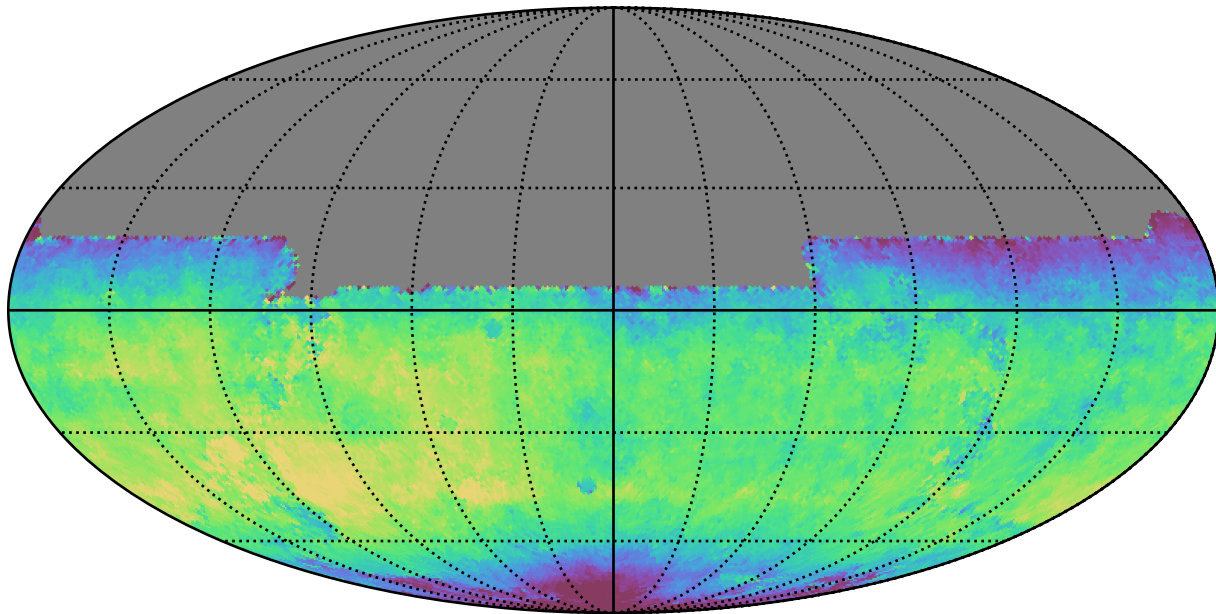
weather_cloudso8v3.4_10yrs All sky y band: Median fiveSigmaDepth
