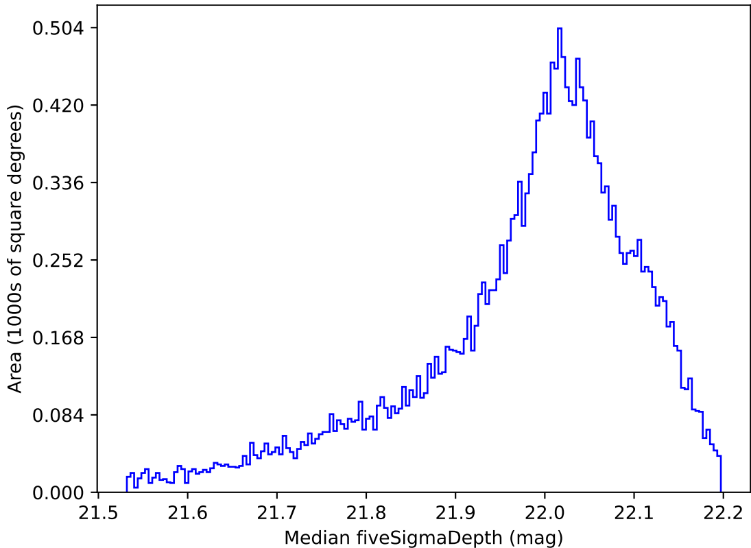
weather_cloudso8v3.4_10yrs All sky y band: Median fiveSigmaDepth
