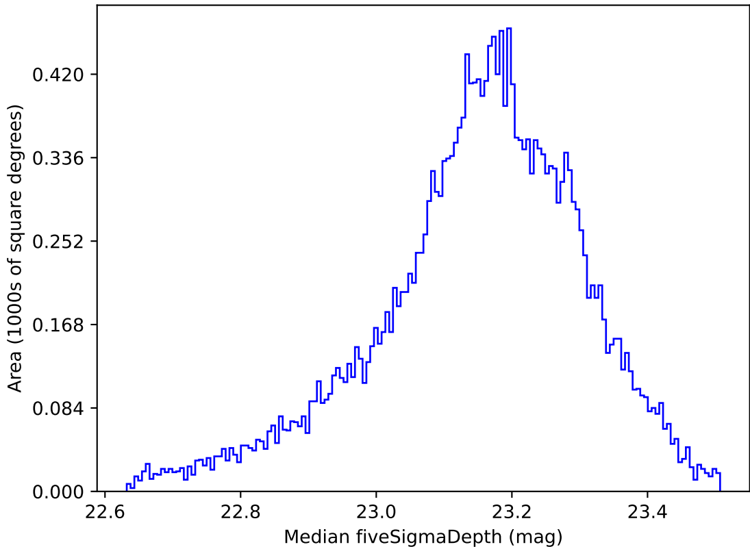
weather_cloudso8v3.4_10yrs All sky u band: Median fiveSigmaDepth
