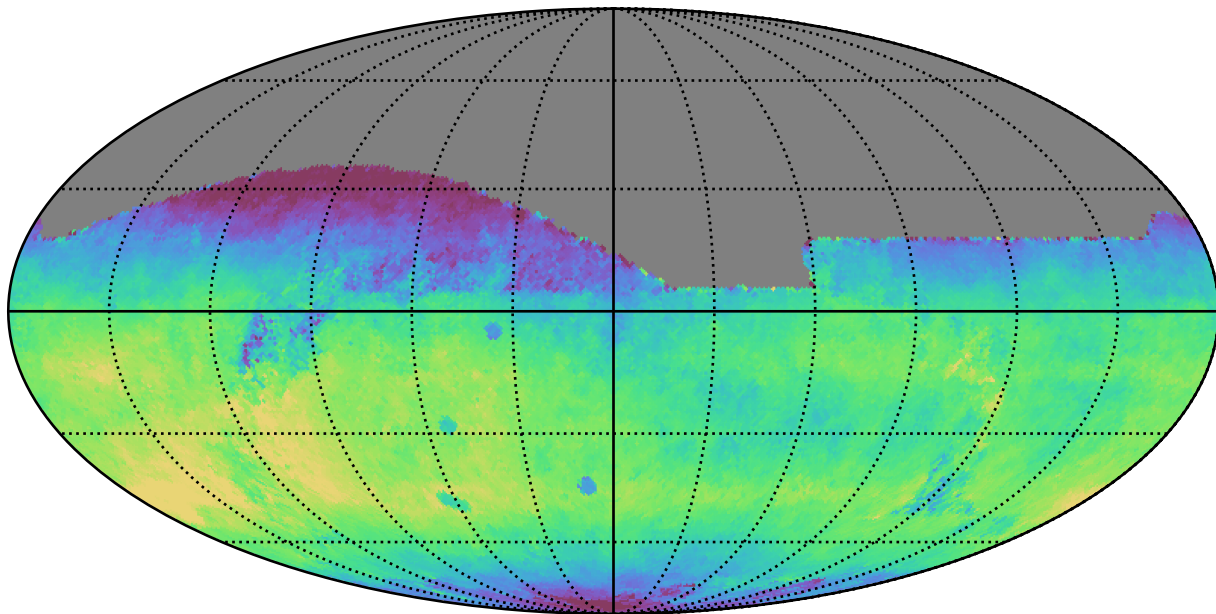
weather_cloudso8v3.4_10yrs All sky r band: Median fiveSigmaDepth
