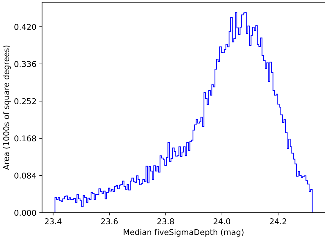
weather_cloudso8v3.4_10yrs All sky r band: Median fiveSigmaDepth
