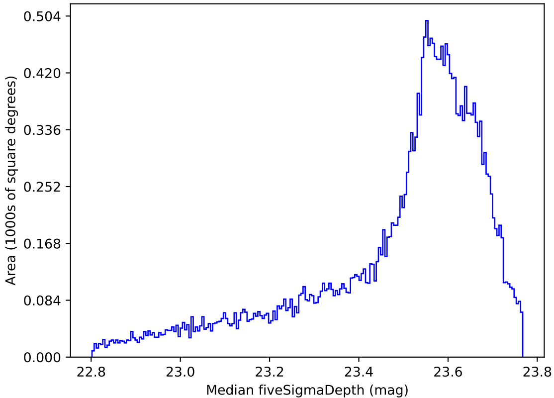
weather_cloudso8v3.4_10yrs All sky i band: Median fiveSigmaDepth
