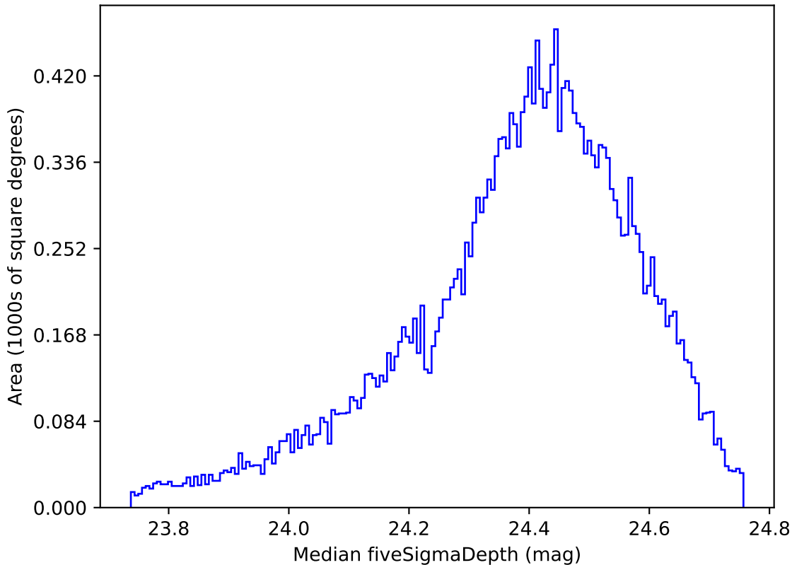
weather_cloudso8v3.4_10yrs All sky g band: Median fiveSigmaDepth
