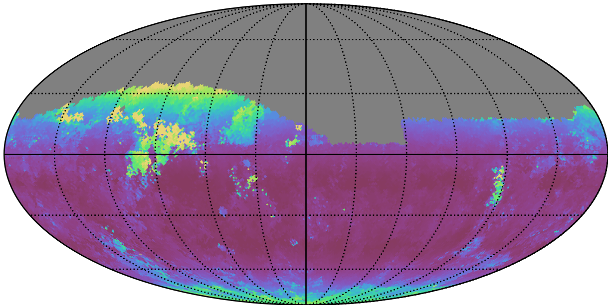
weather_cloudso8v3.4_10yrs Yr 1 z band: Median airmass
