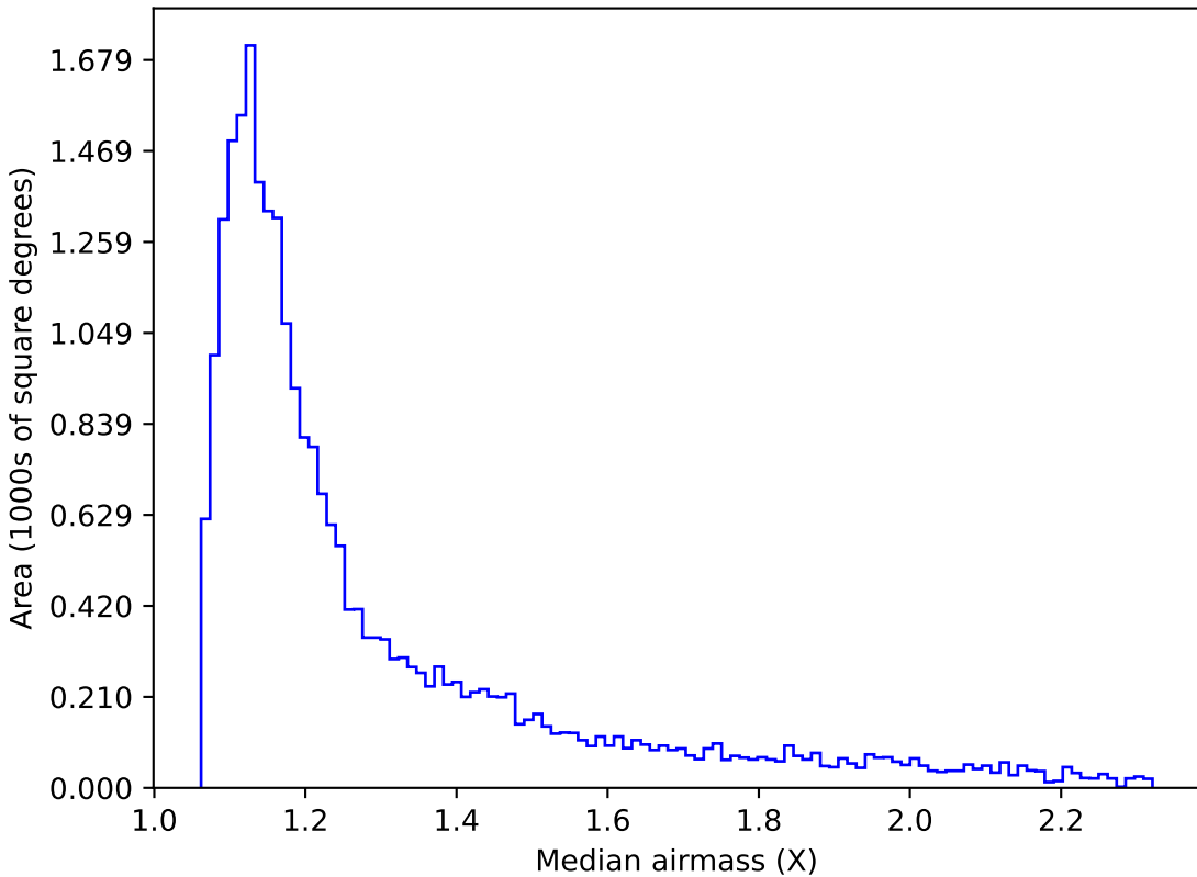
weather_cloudso8v3.4_10yrs Yr 1 z band: Median airmass
