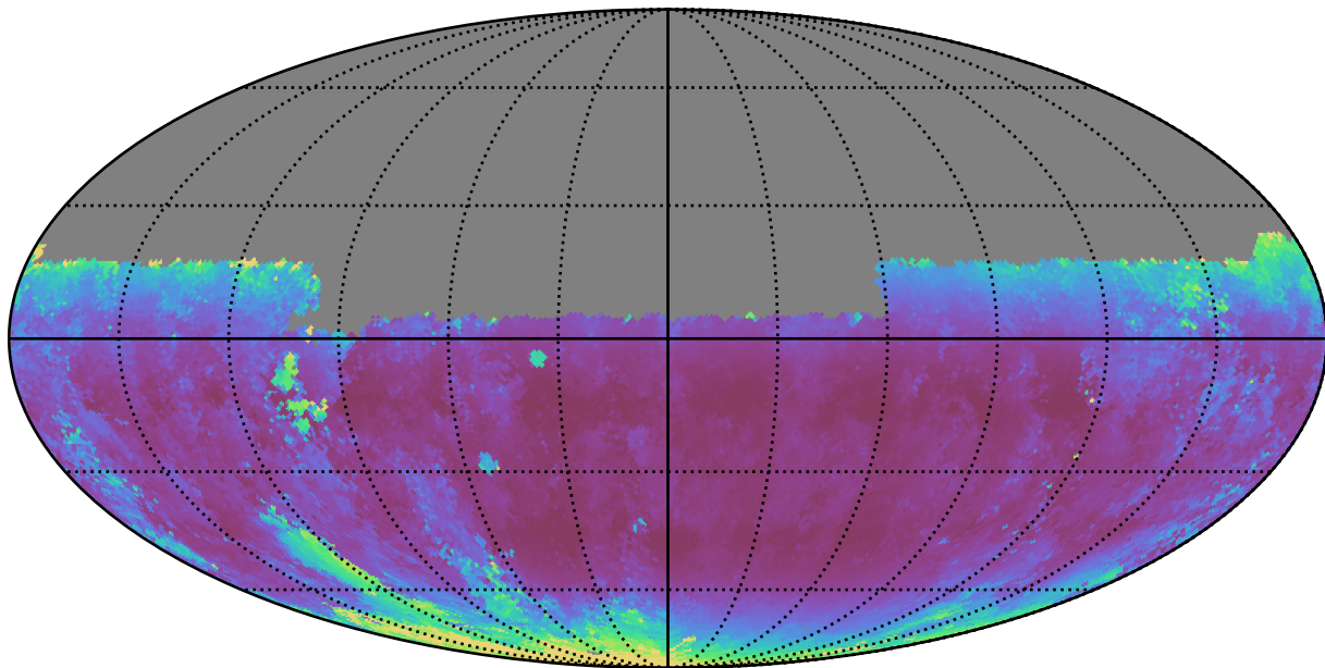
weather_cloudso8v3.4_10yrs Yr 1 y band: Median airmass
