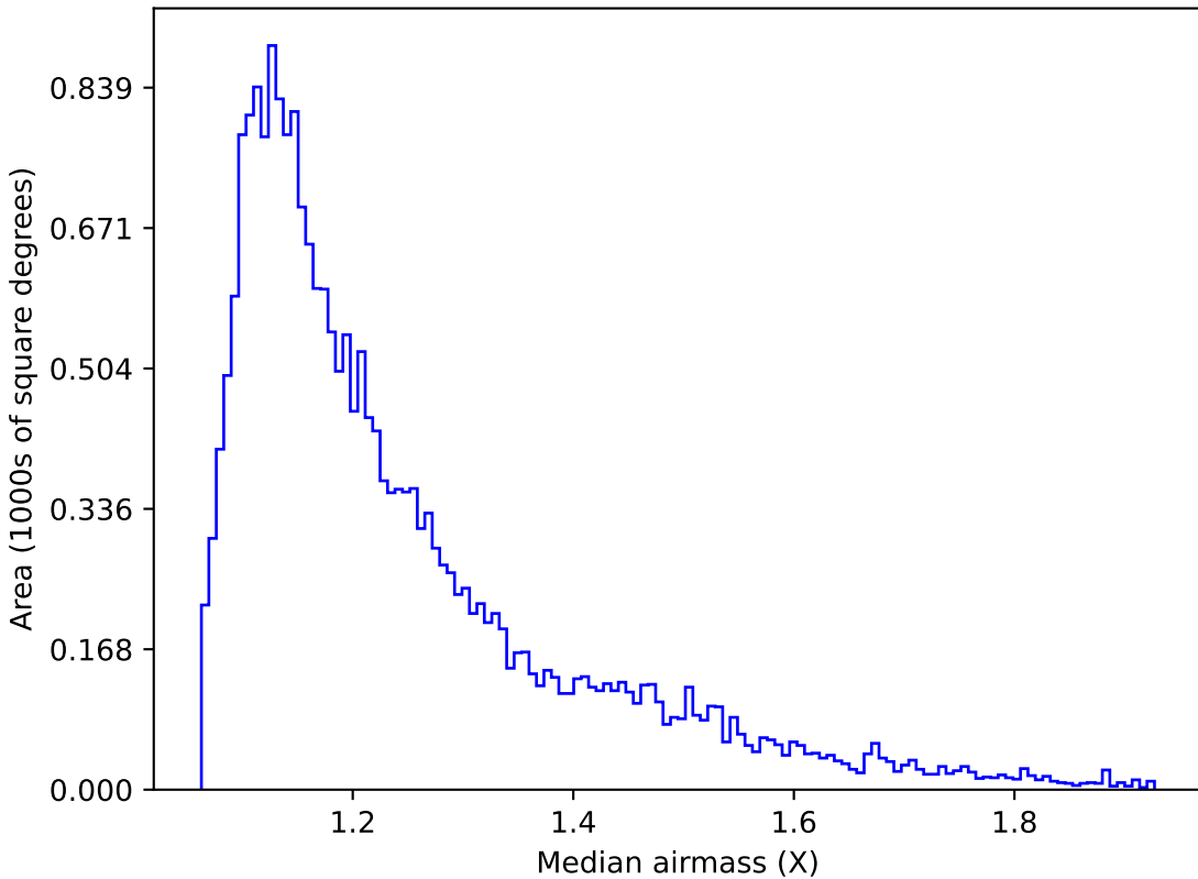
weather_cloudso8v3.4_10yrs Yr 1 y band: Median airmass
