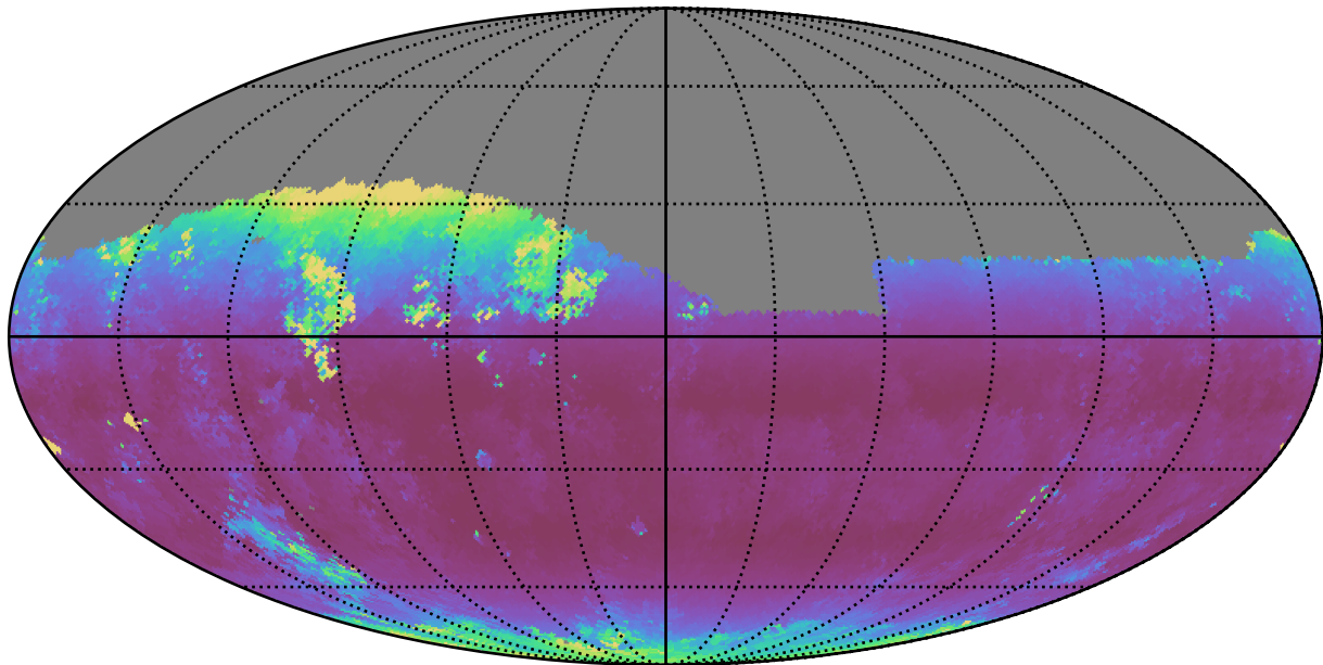
weather_cloudso8v3.4_10yrs Yr 1 i band: Median airmass
