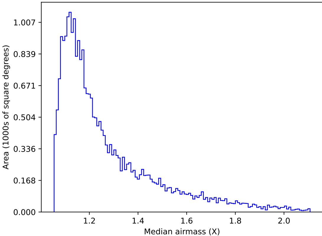
weather_cloudso8v3.4_10yrs Yr 1 g band: Median airmass
