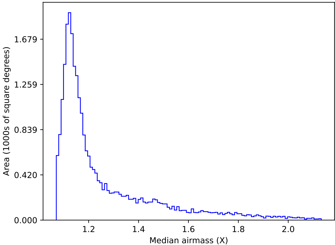
weather_cloudso8v3.4_10yrs Yr 1 all bands: Median airmass
