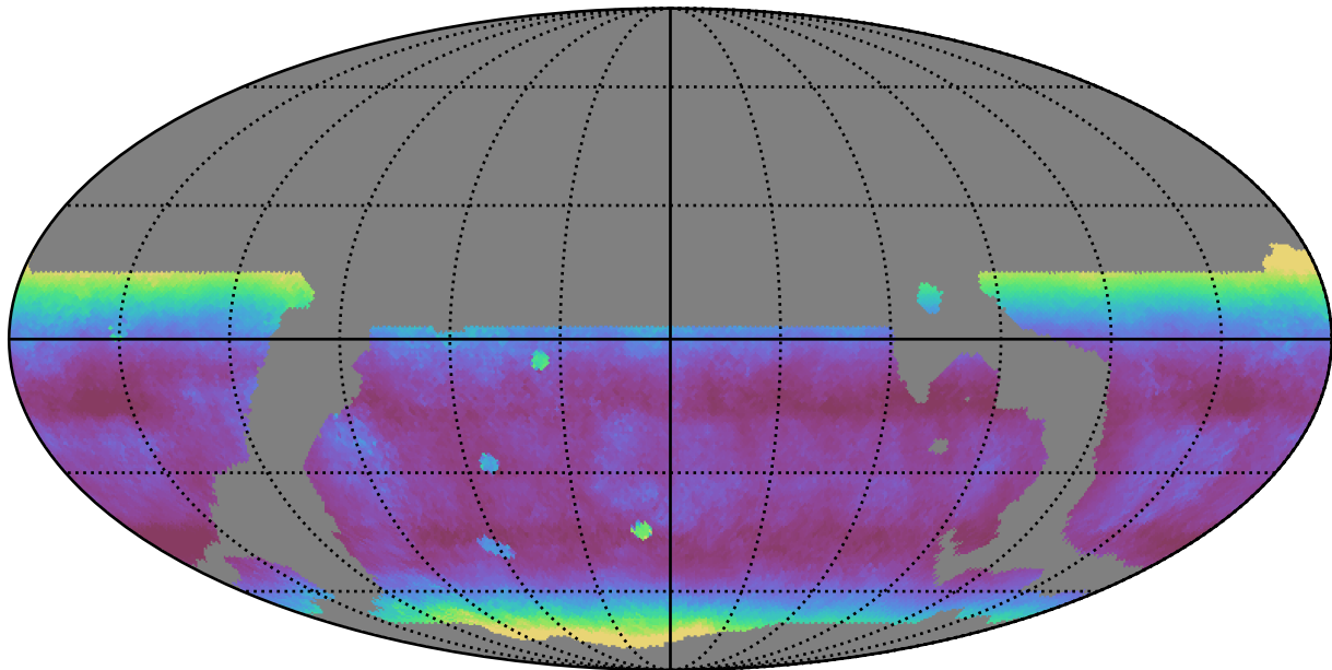
weather_cloudso8v3.4_10yrs WFD z band: Median airmass
