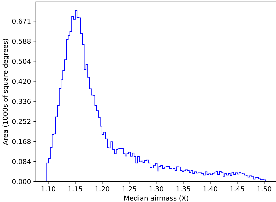
weather_cloudso8v3.4_10yrs WFD z band: Median airmass
