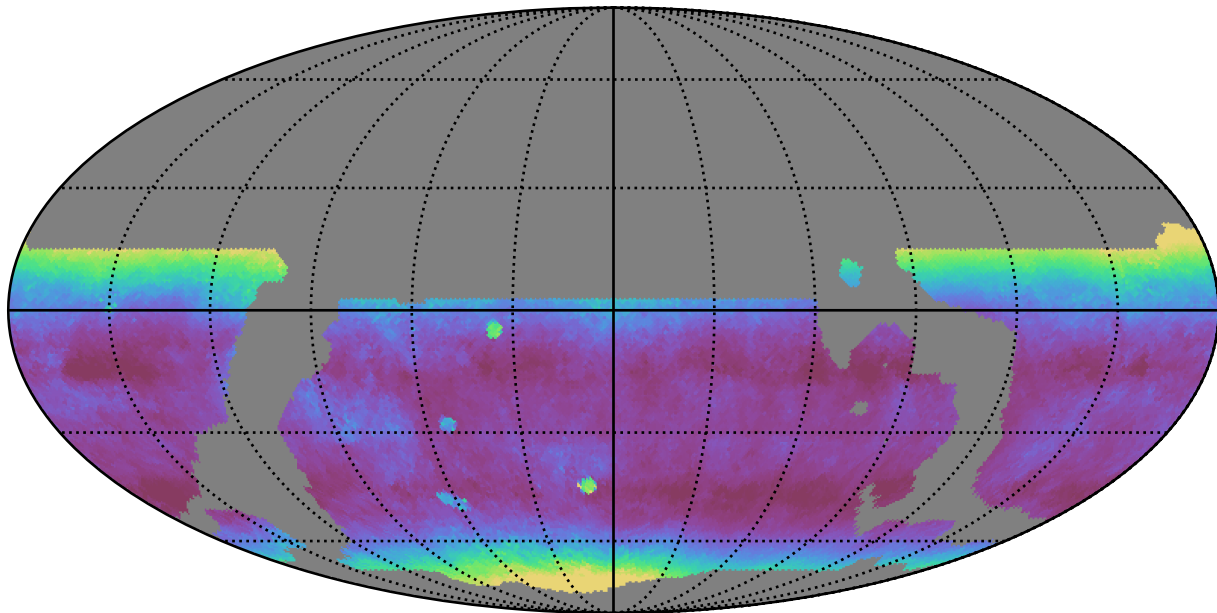
weather_cloudso8v3.4_10yrs WFD y band: Median airmass
