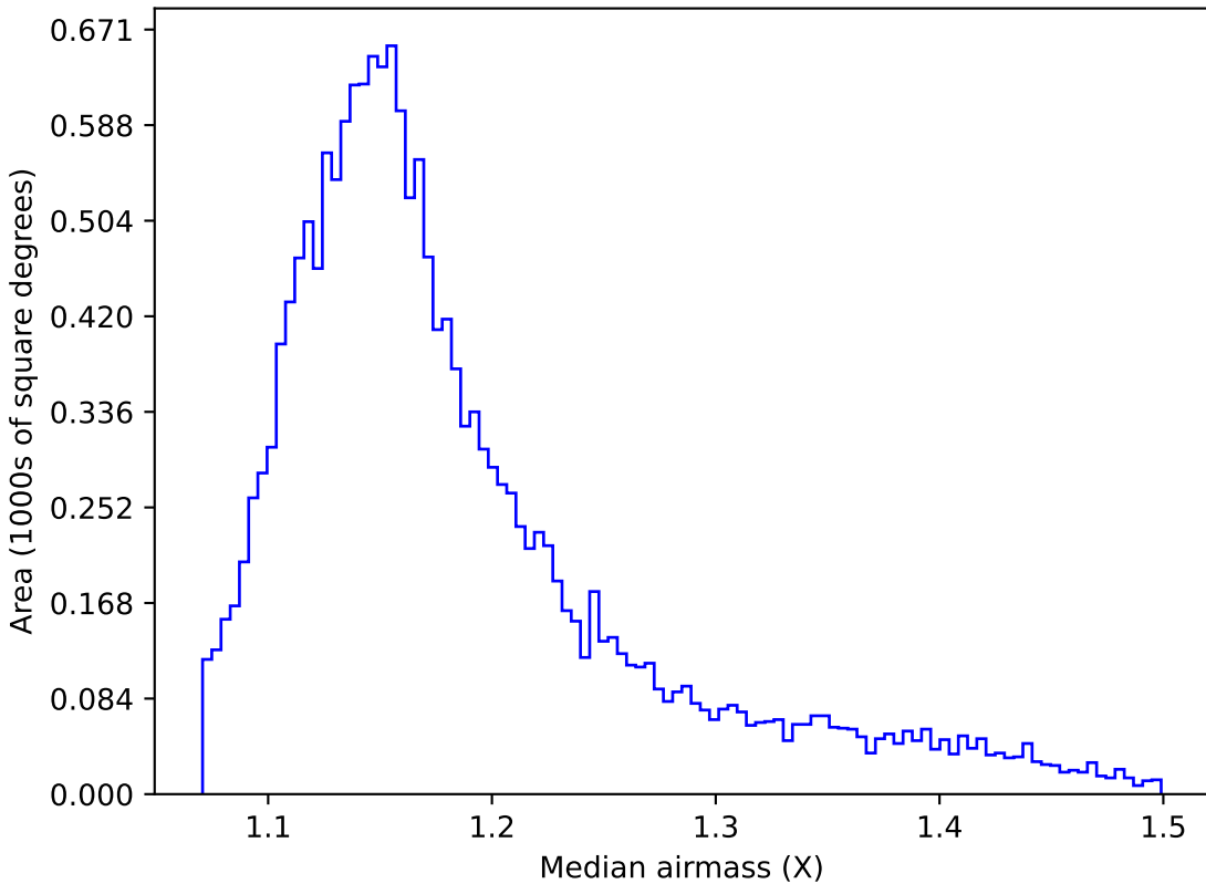
weather_cloudso8v3.4_10yrs WFD u band: Median airmass
