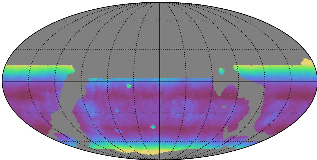
weather_cloudso8v3.4_10yrs WFD r band: Median airmass
