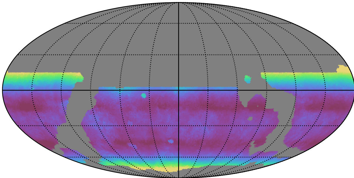
weather_cloudso8v3.4_10yrs WFD i band: Median airmass
