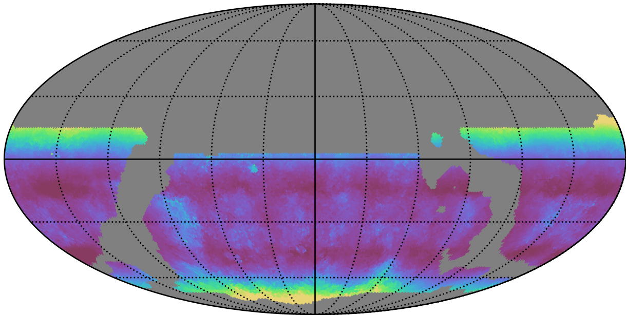
weather_cloudso8v3.4_10yrs WFD g band: Median airmass
